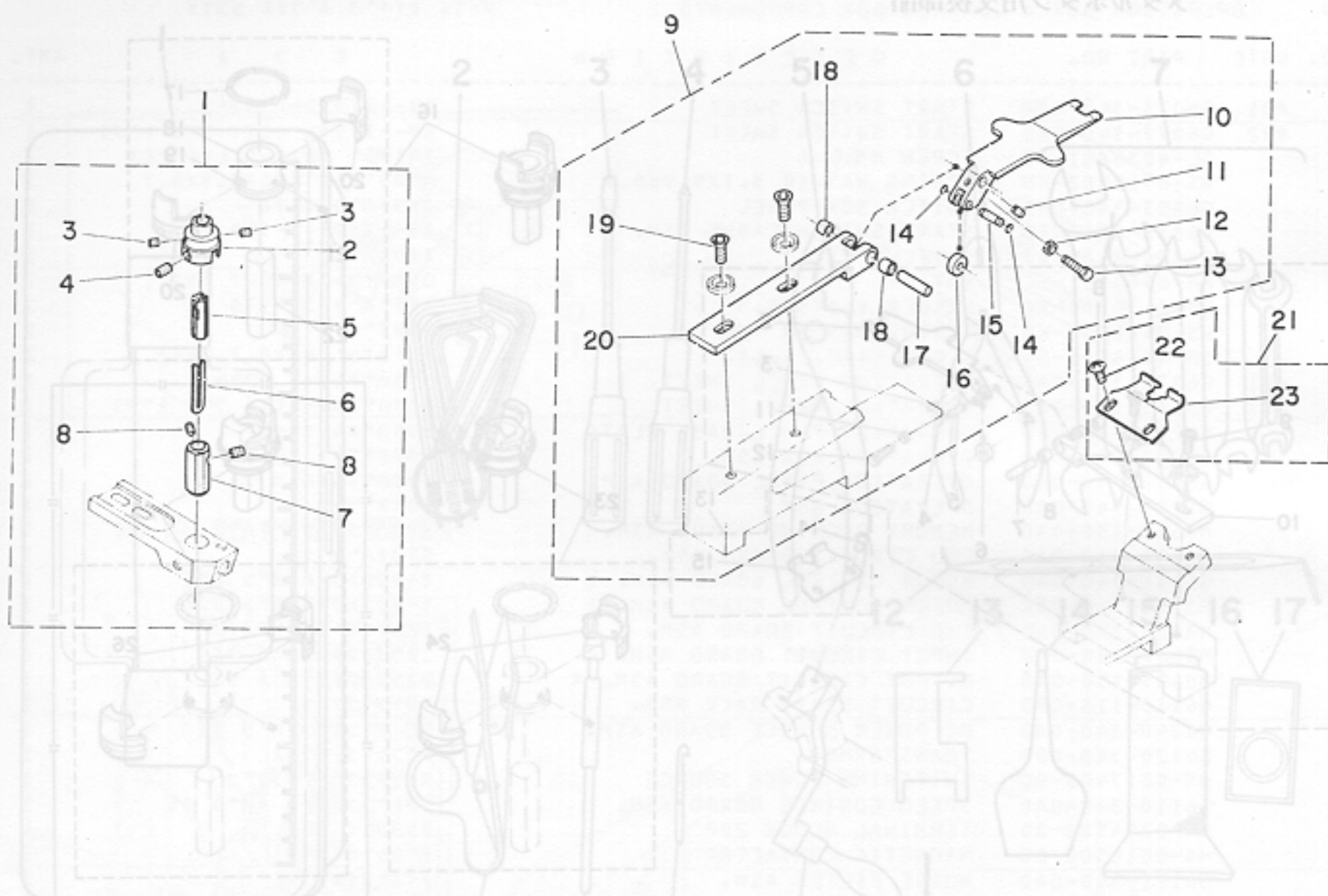
22 S-124: EXCHANGING PARTS FOR 2-HOLED BUTTON
