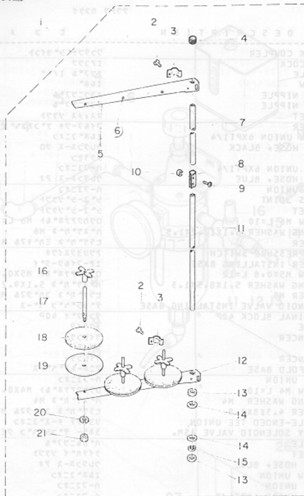
17 THREAD STAND UNIT
