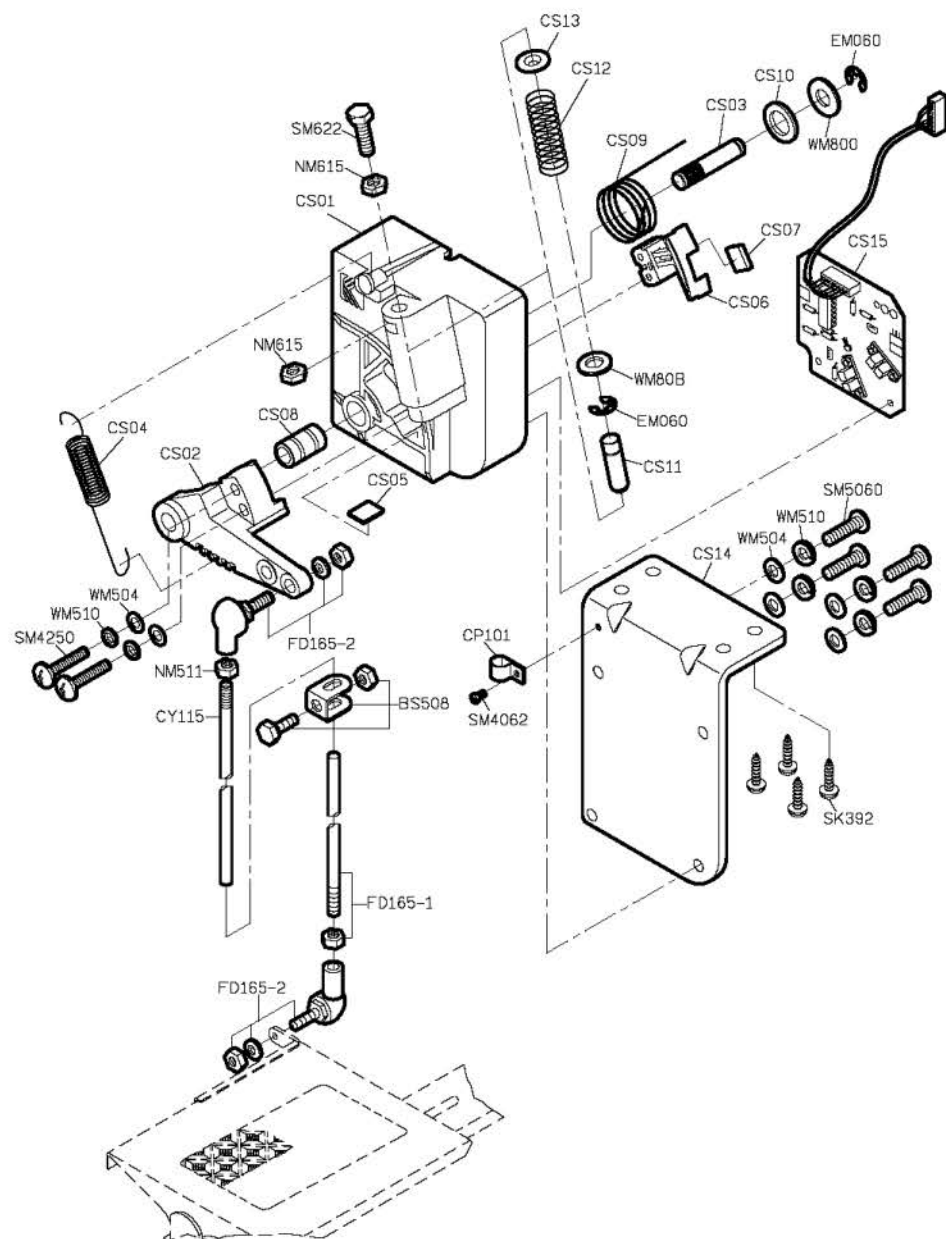
PARTS LIST FOR CS GROUP
