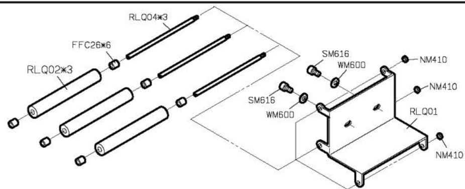
PARTS LIST FOR RLQ GROUP
