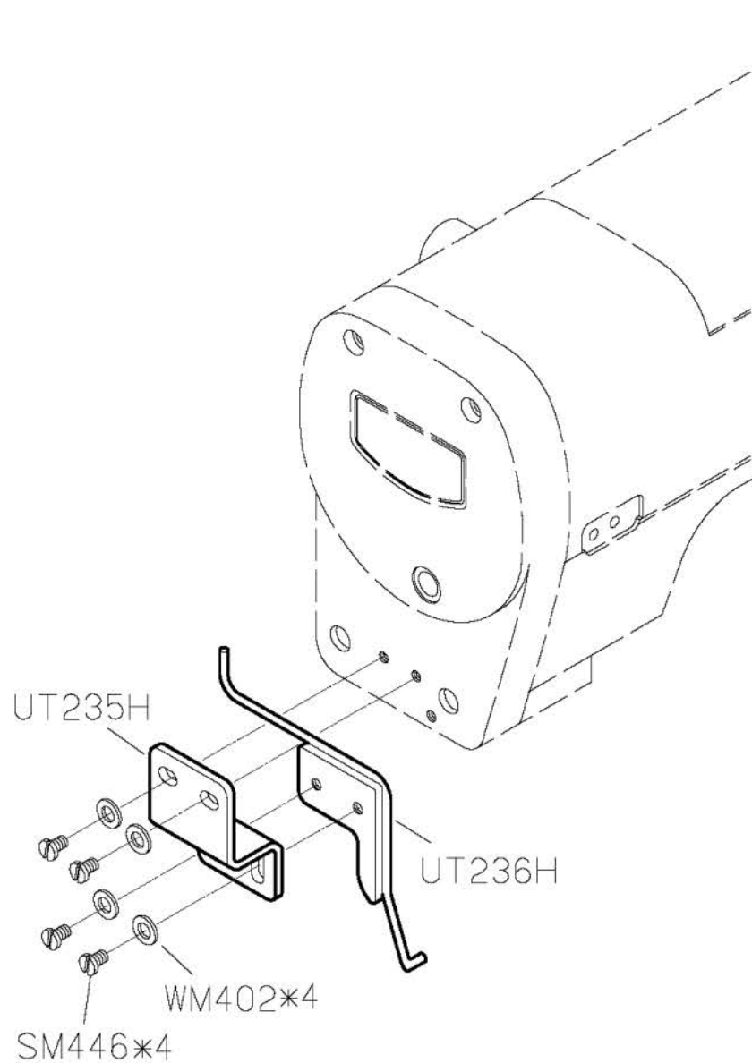
PARTS LIST FOR UTP/UTQ GROUP
