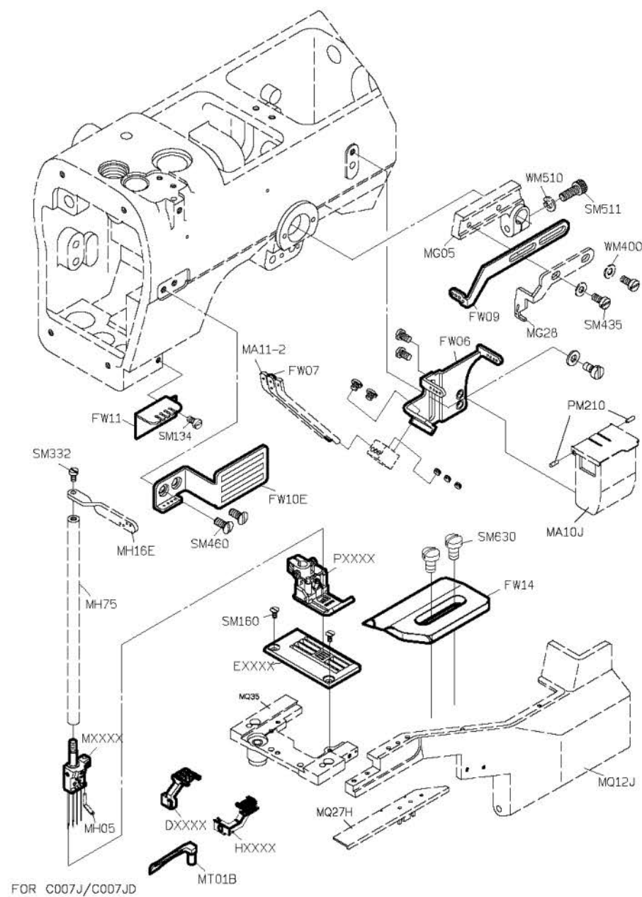
PARTS LIST FOR CW GROUP
